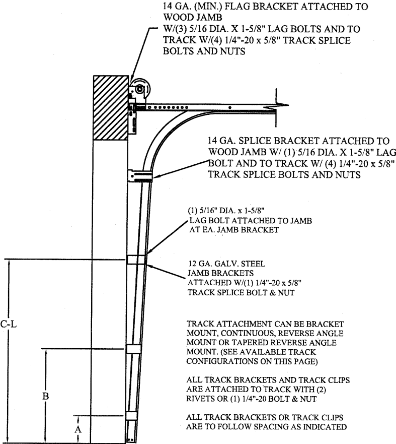
TRACK CONFIGURATION FOR UP TO 24' TALL DOORS SEE TABLE 2
